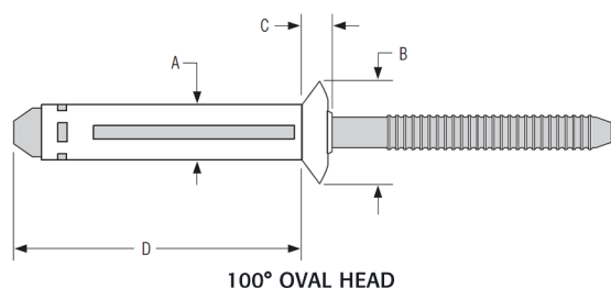
100° OVAL HEAD
