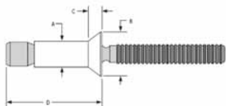
100° COUNTERSUNK HEAD
