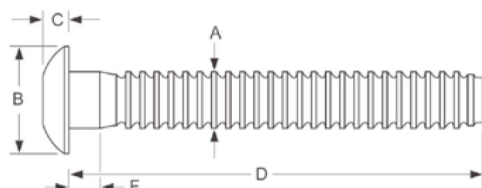
TRUSS HEAD
