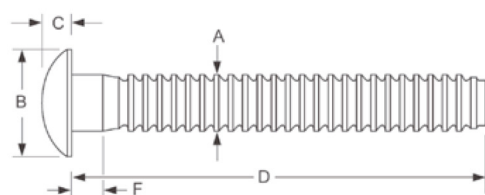
RIVET HEAD
