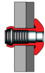
AFTER INSTALLATION
