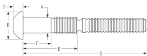
ROUND HEAD
