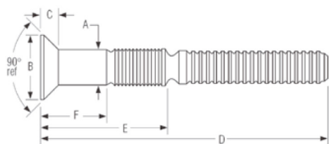
COUNTERSUNK HEAD
